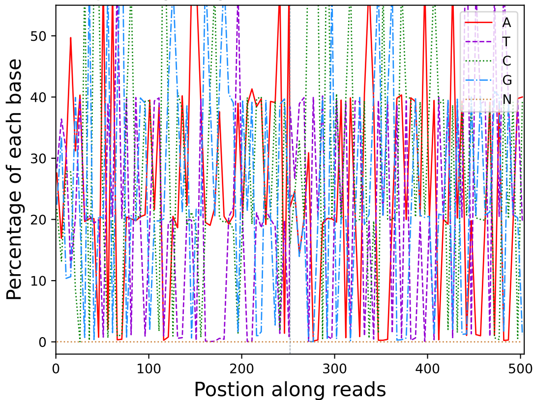
Base percentage along reads (R10806)
